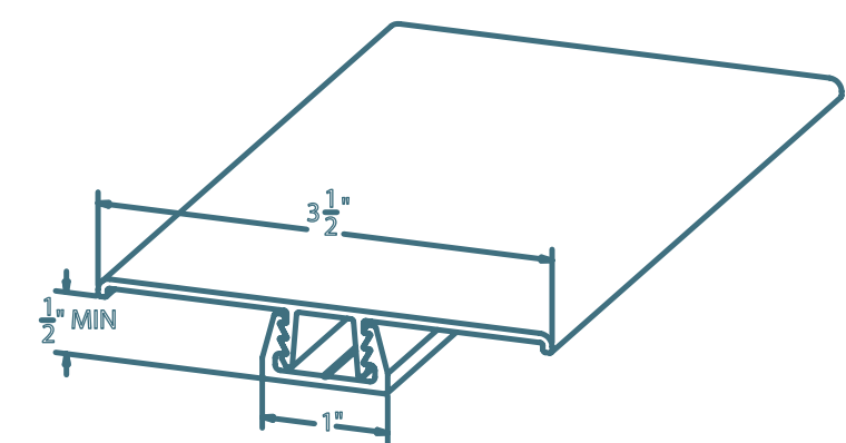
Snap-In H Trim
