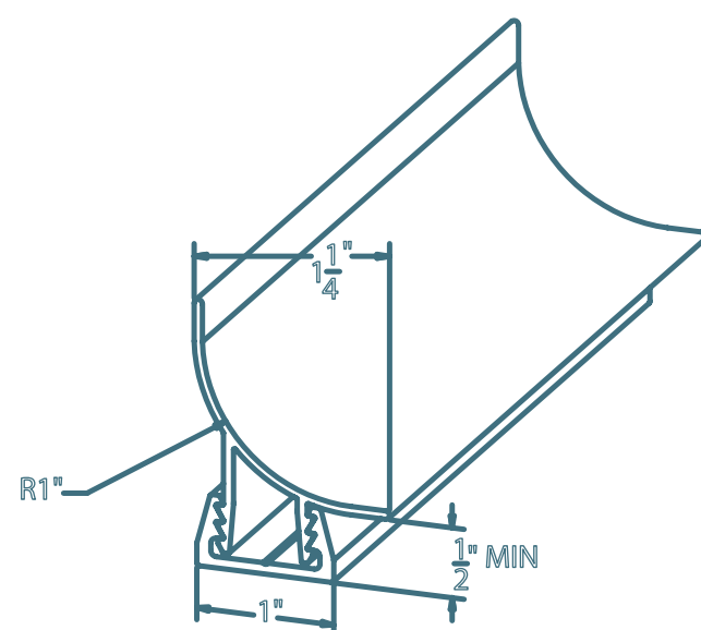
Snap-In Inside Cove
